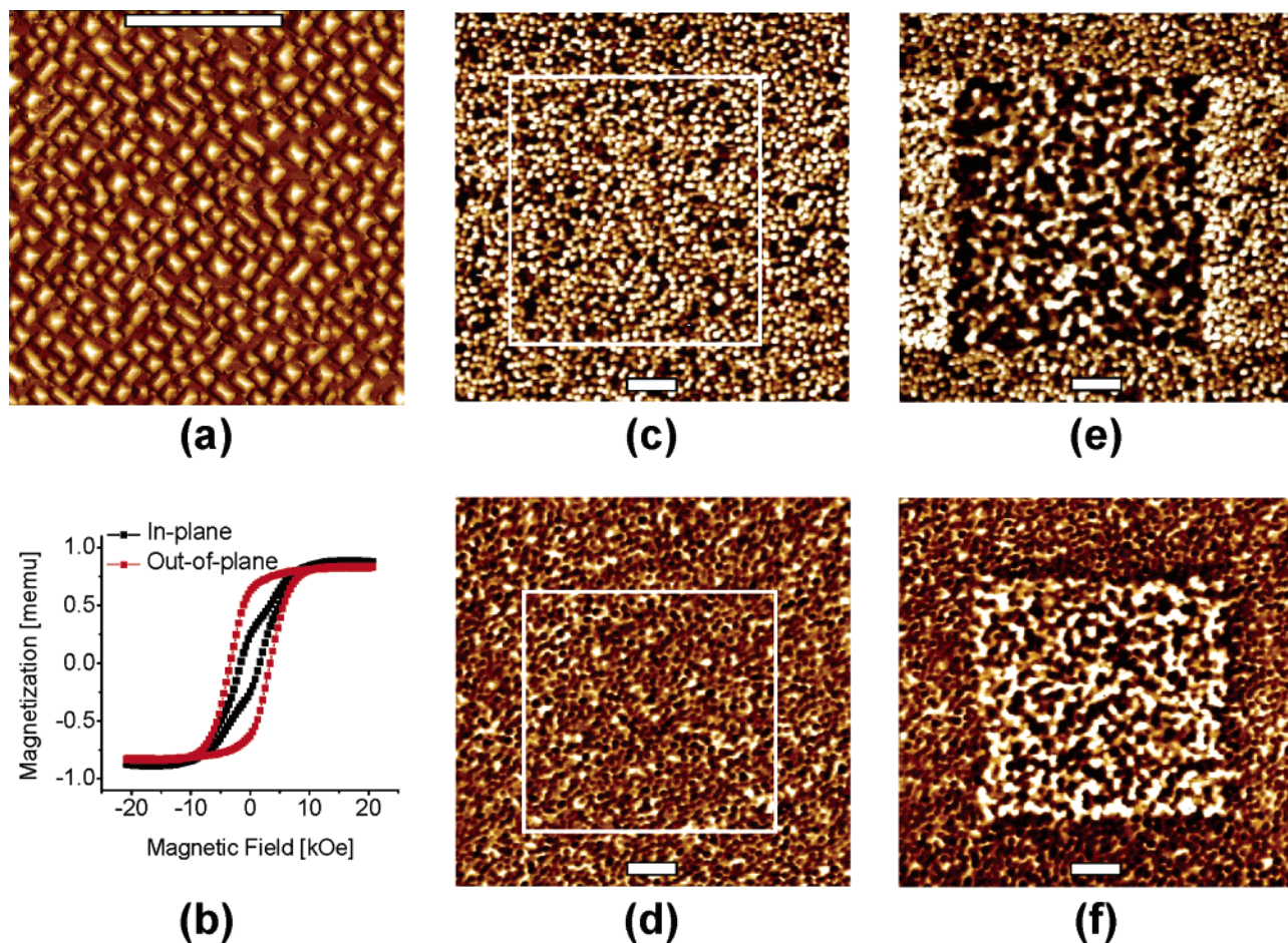
Figure 1. Morphology and magnetization switching in the (\text{BiFeO}_3)_{0.65}-(\text{CoFe}_2\text{O}_4)_{0.35} nanostructure. (a) Surface topography as seen by AFM. (b) Out-of-plane (red symbols) and in-plane (black symbols) magnetization loops. (c,d) MFM scans after magnetization in down and up 20 kOe fields, respectively. (e,f) MFM scans taken in the same areas as in (c) and (d), respectively, after electrical poling at -16 V. The bars are 1\ \mu\text{m} .
